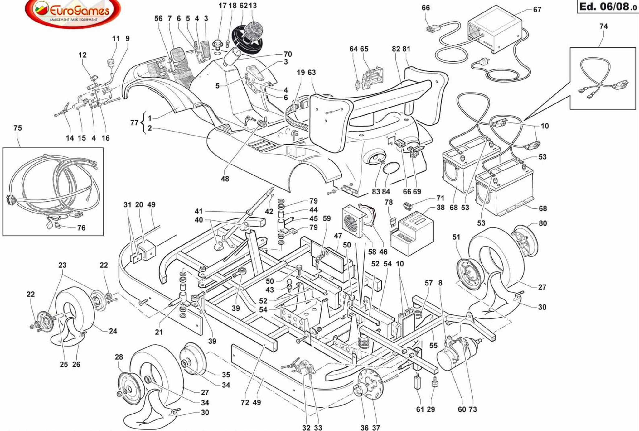
Mod. GO KART DOUBLE Cod. 6850
